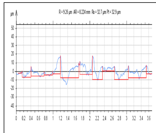
Fig 14: V=565.74m/min,F=32mm/min.,D=0.75mm
