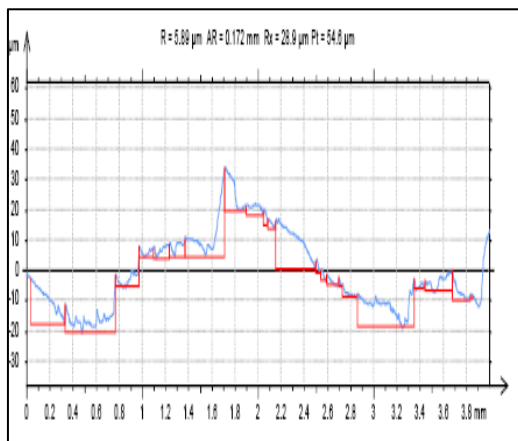
Fig 5: V=565.74m/min,F=32mm/min.,D=0.5mm
