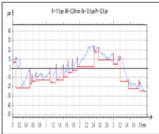
Fig 5: V=565.74m/min,F=32mm/min.,D=0.5mm
