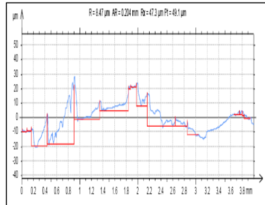
Fig 13: V=565.74 m/min,F=20mm/min.,D=0.75mm
