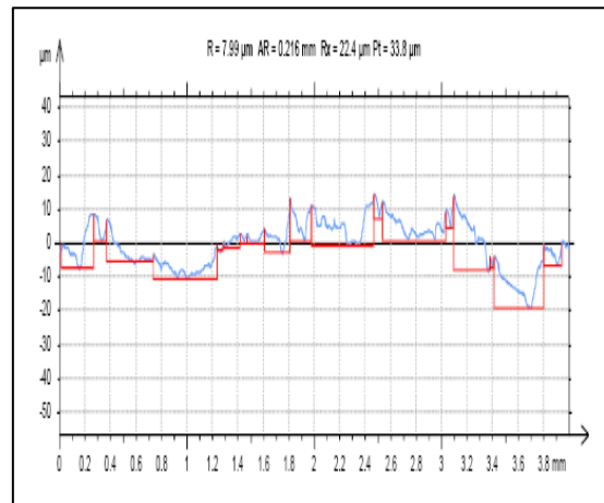
Fig 14: V=565.74m/min,F=32mm/min.,D=0.75mm
